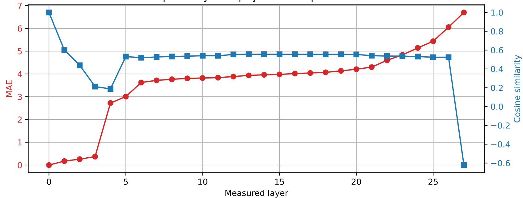
Qwen2.5-7B-Instruct | Prompt 3 Spared layer 21 | Hybrid vs unquantized
