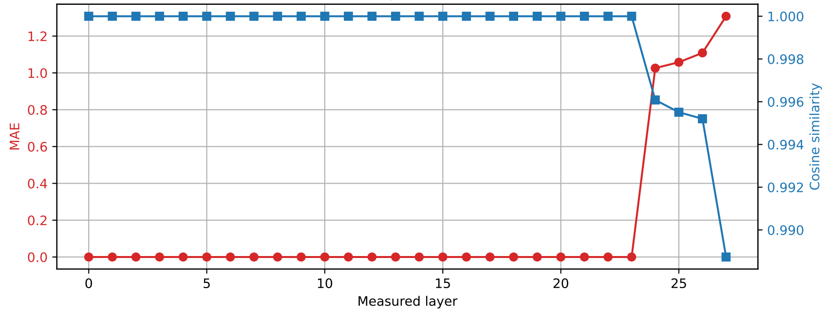
Qwen2.5-7B-Instruct | Prompt 3 Spared layer 23 | Hybrid vs quantized
