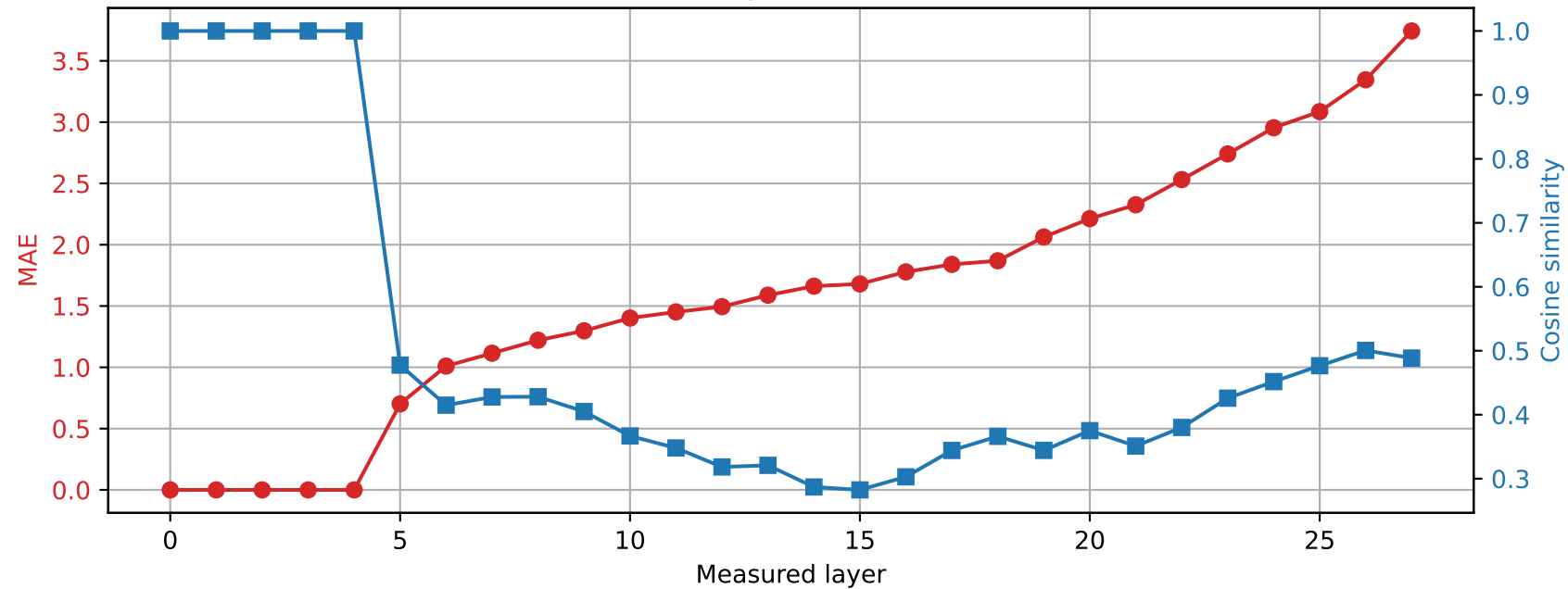
Qwen2.5-7B-Instruct | Prompt 4 Spared layer 4 | Hybrid vs quantized
