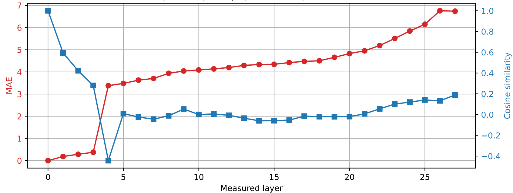
Qwen2.5-7B-Instruct | Prompt 4 Spared layer 7 | Hybrid vs unquantized
