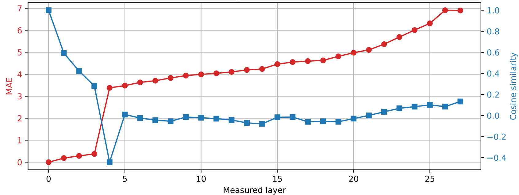
Qwen2.5-7B-Instruct | Prompt 4 Spared layer 14 | Hybrid vs unquantized
