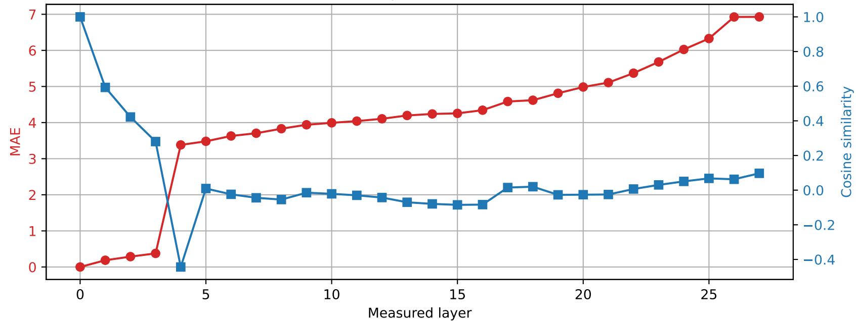
Qwen2.5-7B-Instruct | Prompt 4 Spared layer 16 | Hybrid vs unquantized
