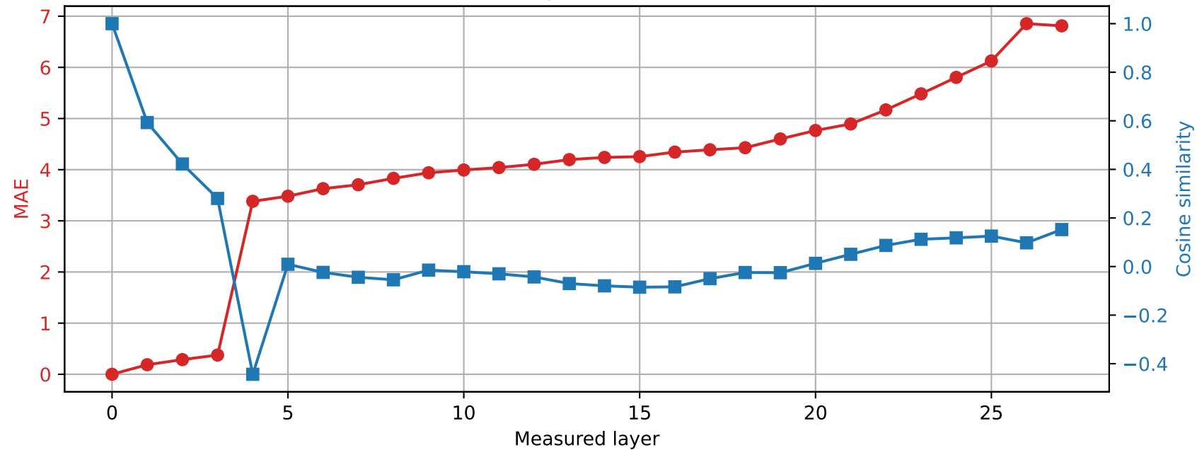
Qwen2.5-7B-Instruct | Prompt 4 Spared layer 25 | Hybrid vs unquantized
