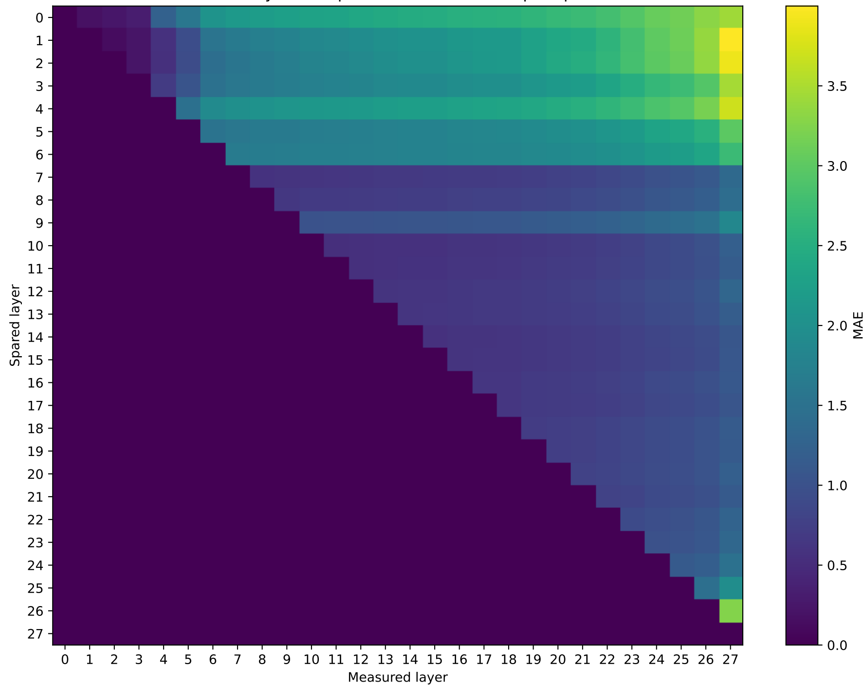
Qwen2.5-7B-Instruct Mean hybrid vs quantized MAE across 5 prompts
