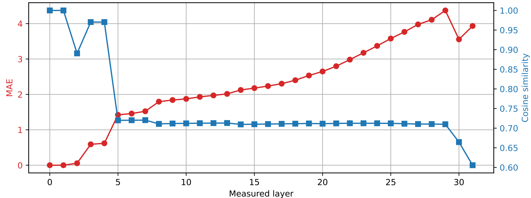
Phi-3-mini-4k-instruct | Prompt 0 Spared layer 0 | Hybrid vs unquantized
