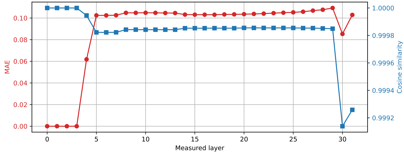
Phi-3-mini-4k-instruct | Prompt 0 Spared layer 3 | Hybrid vs quantized
