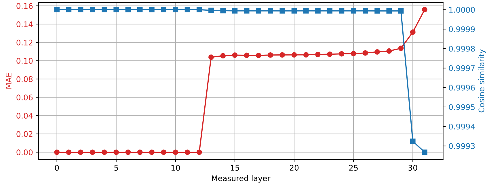
Phi-3-mini-4k-instruct | Prompt 0 Spared layer 12 | Hybrid vs quantized
