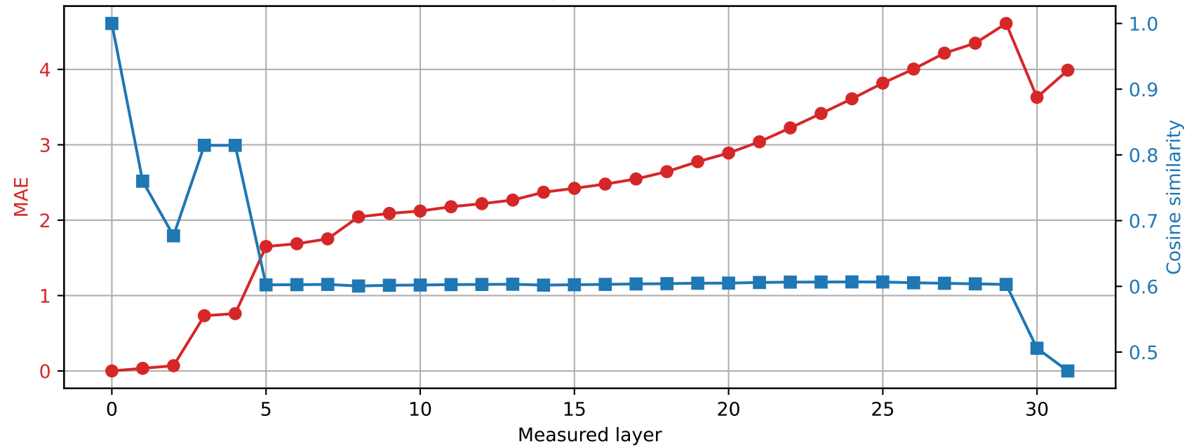
Phi-3-mini-4k-instruct | Prompt 0 Spared layer 12 | Hybrid vs unquantized
