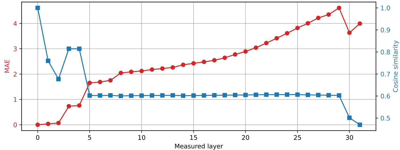
Phi-3-mini-4k-instruct | Prompt 0 Spared layer 14 | Hybrid vs unquantized
