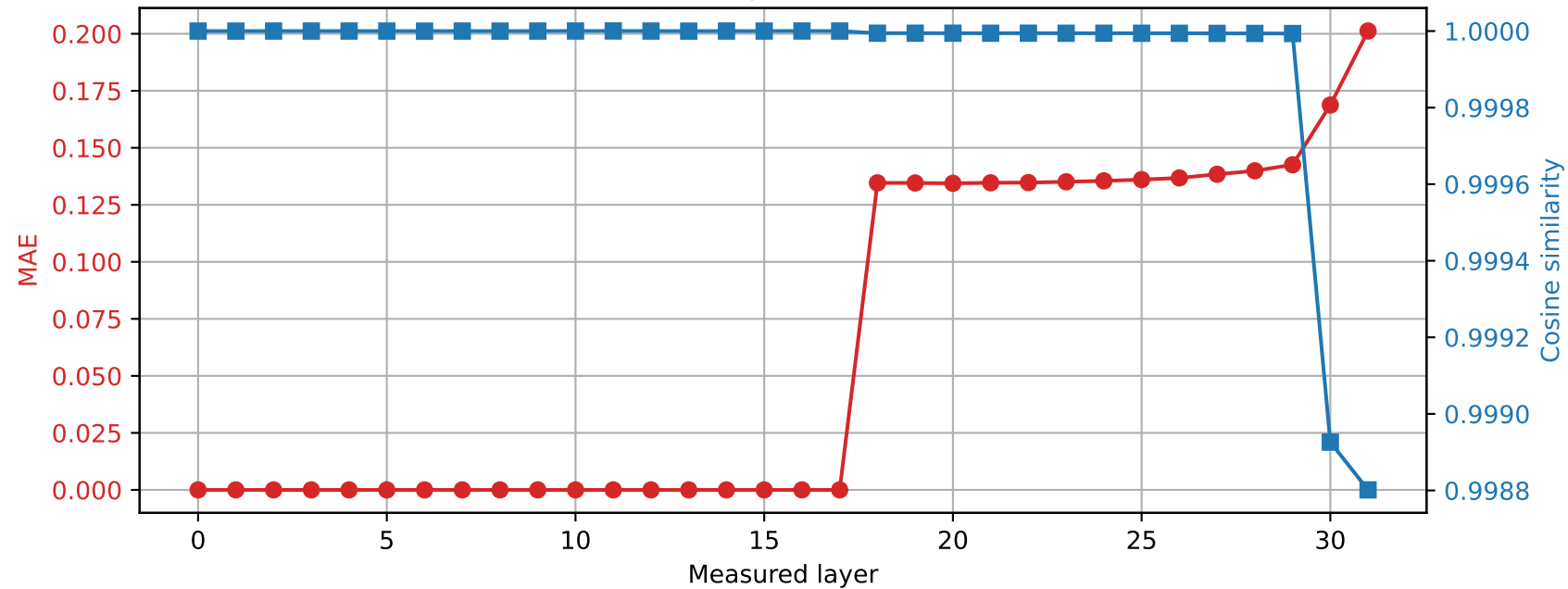
Phi-3-mini-4k-instruct | Prompt 0 Spared layer 17 | Hybrid vs quantized
