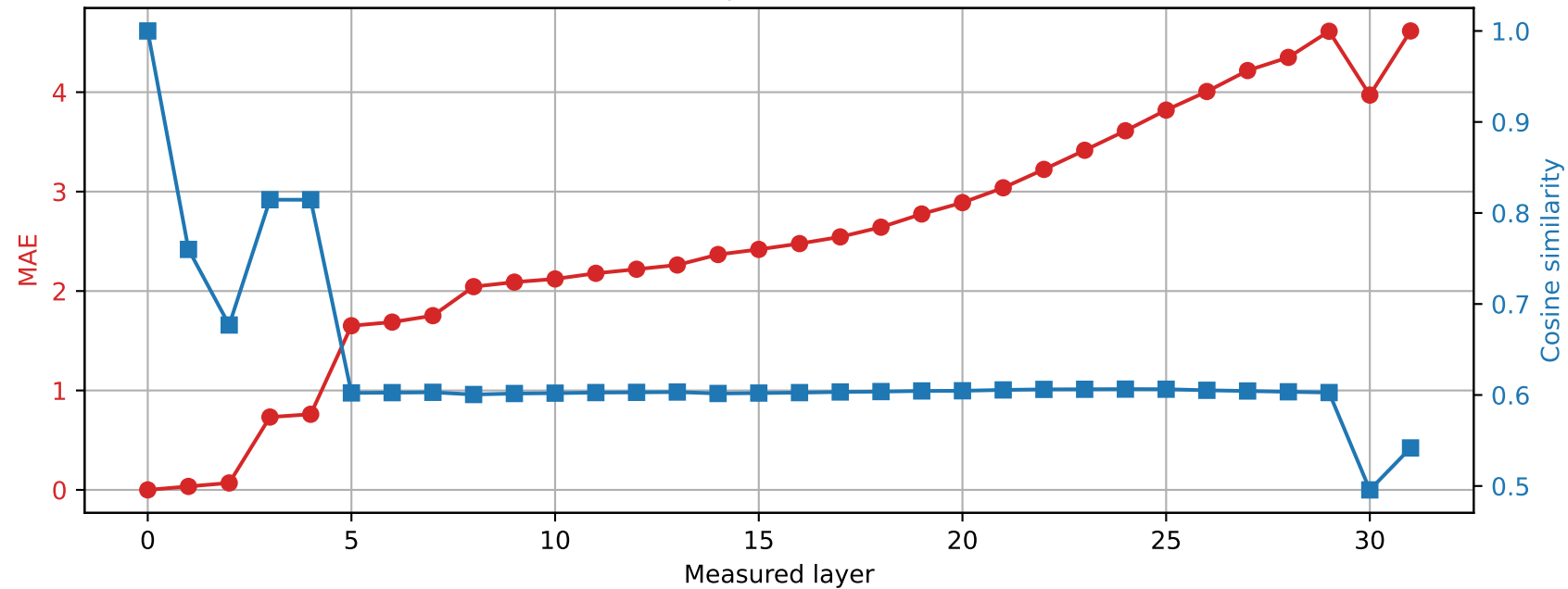
Phi-3-mini-4k-instruct | Prompt 0 Spared layer 29 | Hybrid vs unquantized
