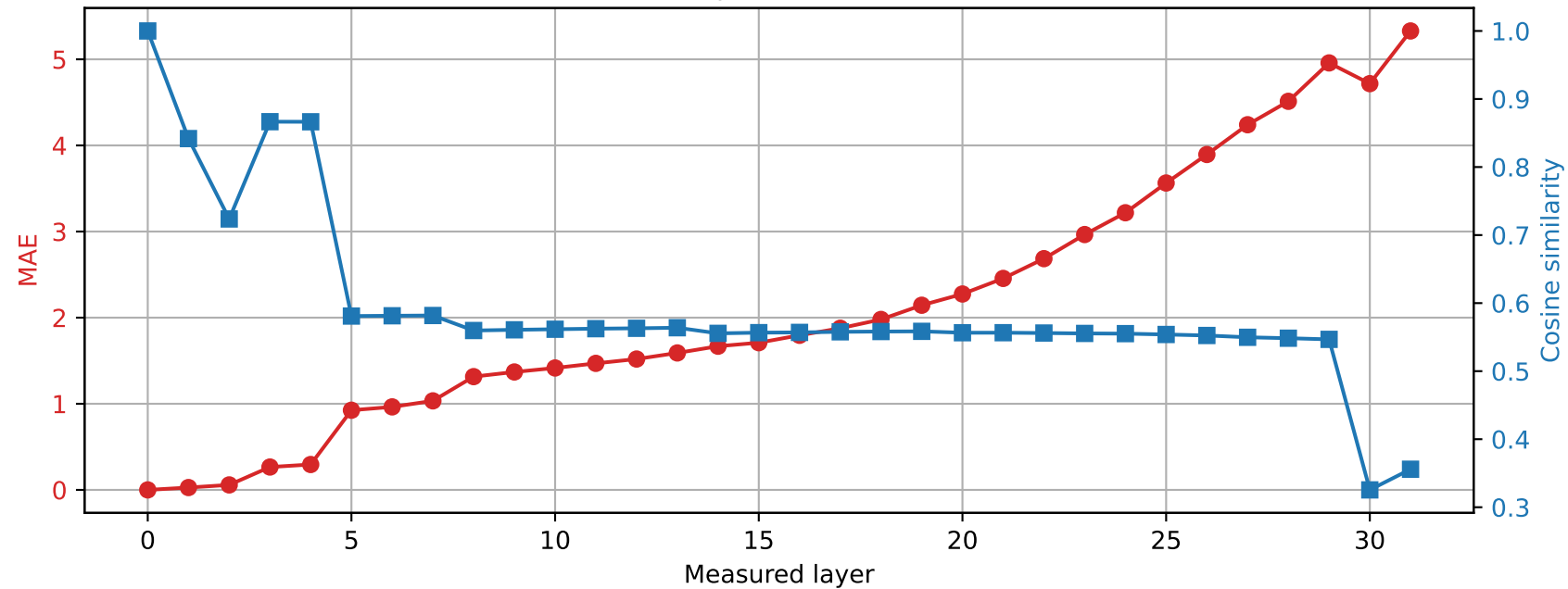
Phi-3-mini-4k-instruct | Prompt 1 Spared layer 7 | Hybrid vs unquantized
