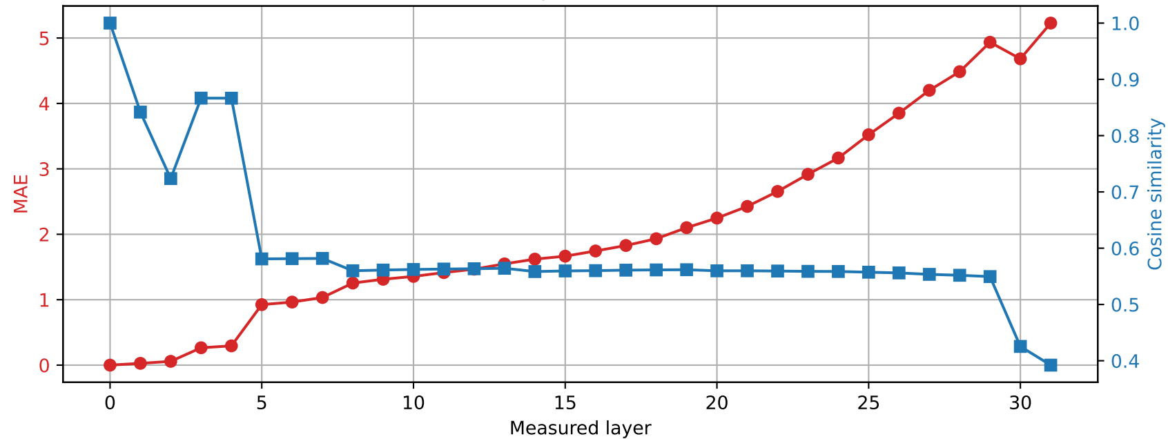
Phi-3-mini-4k-instruct | Prompt 1 Spared layer 15 | Hybrid vs unquantized
