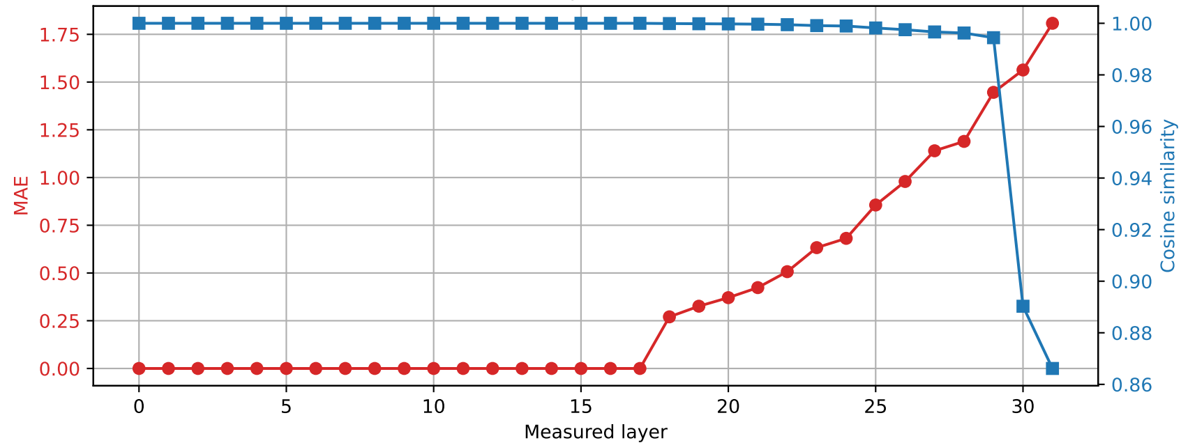
Phi-3-mini-4k-instruct | Prompt 1 Spared layer 17 | Hybrid vs quantized
