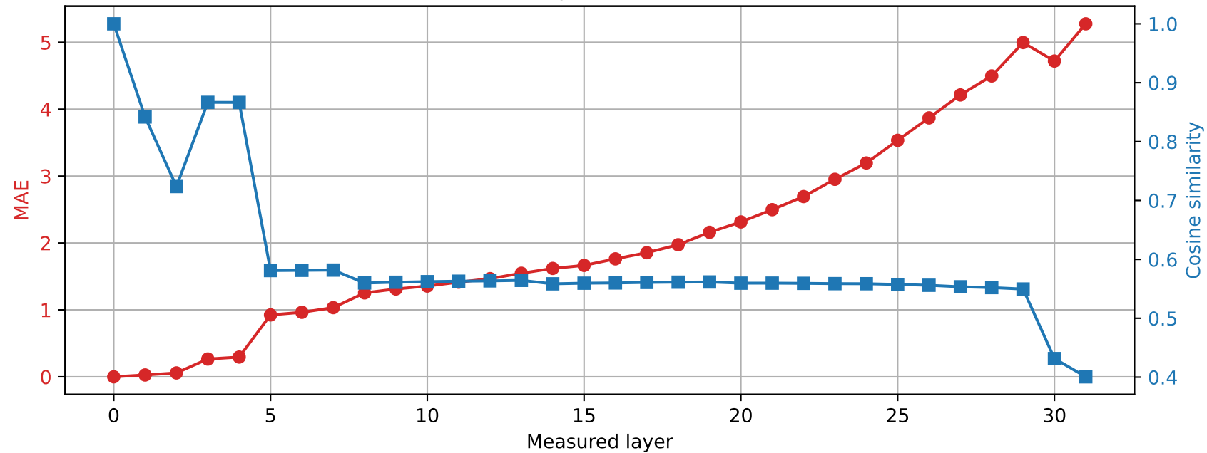
Phi-3-mini-4k-instruct | Prompt 1 Spared layer 21 | Hybrid vs unquantized
