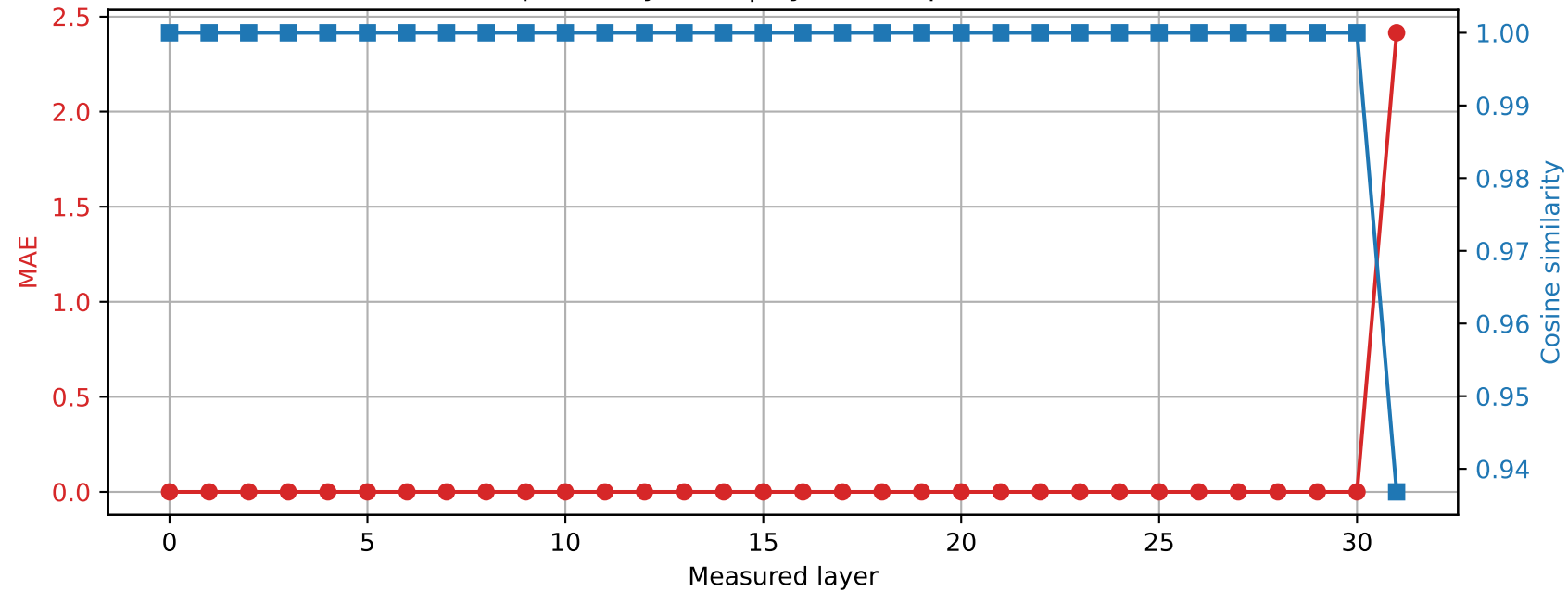
Phi-3-mini-4k-instruct | Prompt 1 Spared layer 30 | Hybrid vs quantized
