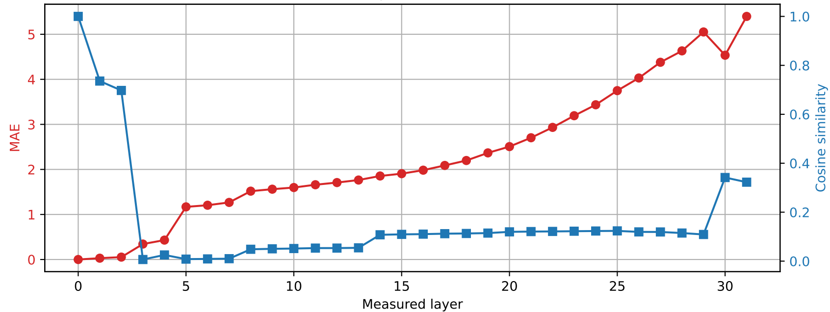
Phi-3-mini-4k-instruct | Prompt 2 Spared layer 3 | Hybrid vs unquantized
