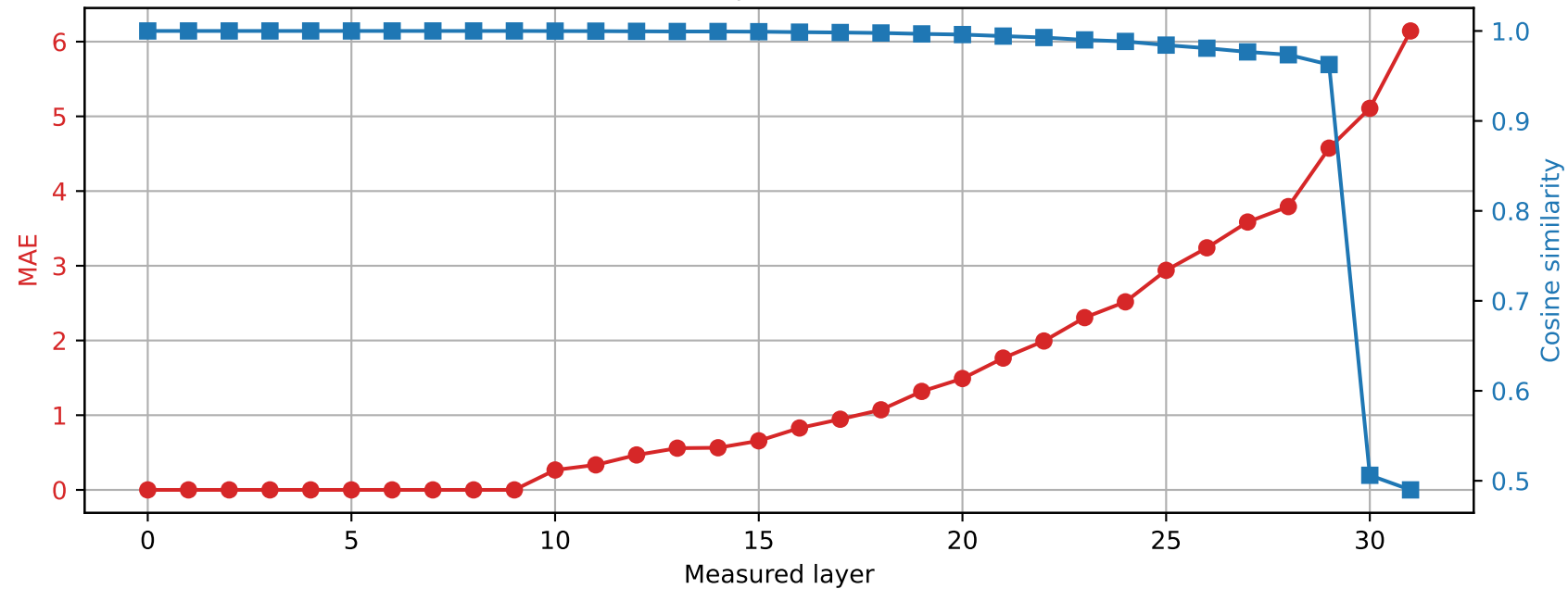
Phi-3-mini-4k-instruct | Prompt 2 Spared layer 9 | Hybrid vs quantized
