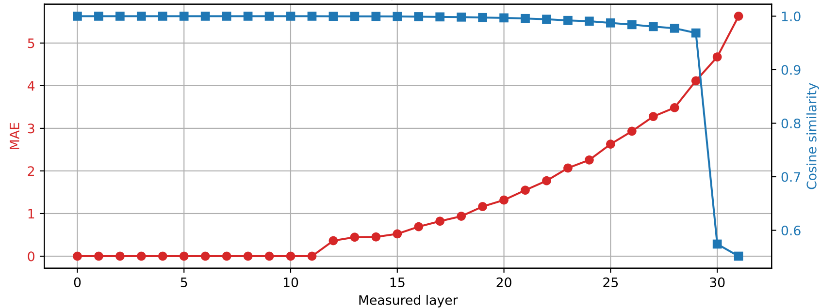
Phi-3-mini-4k-instruct | Prompt 2 Spared layer 11 | Hybrid vs quantized
