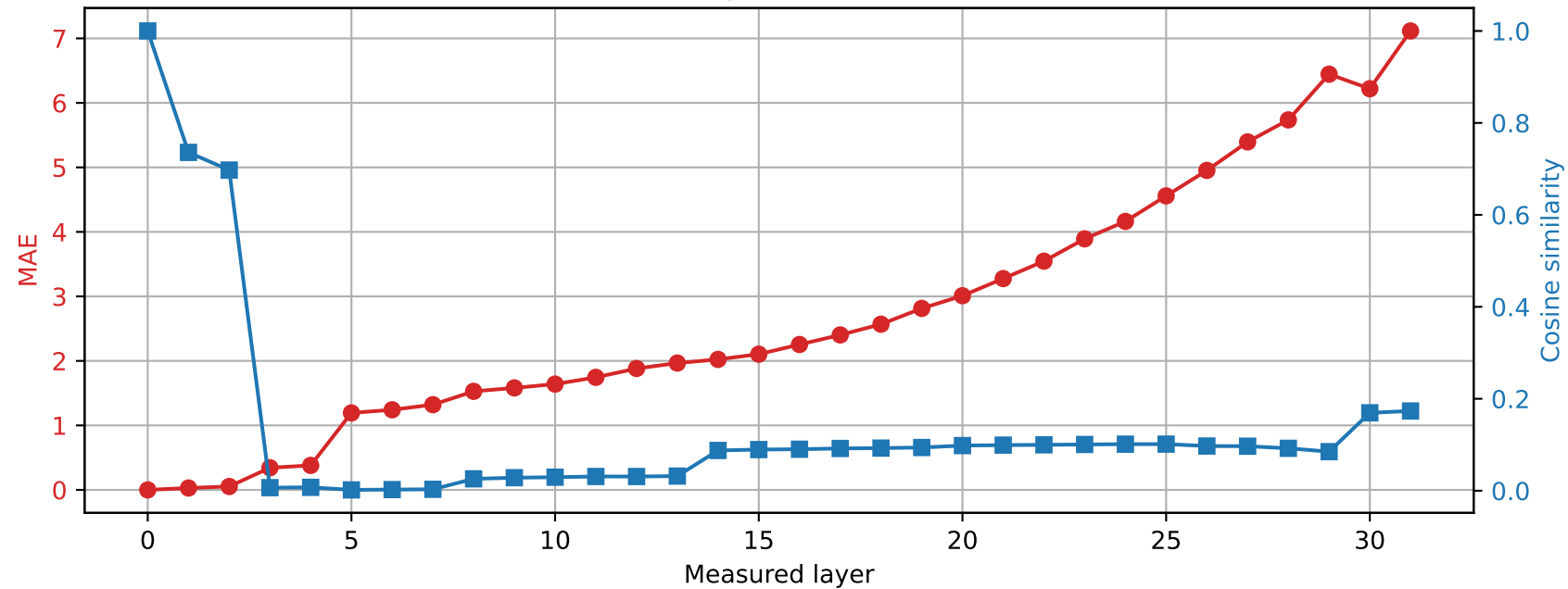
Phi-3-mini-4k-instruct | Prompt 2 Spared layer 11 | Hybrid vs unquantized
