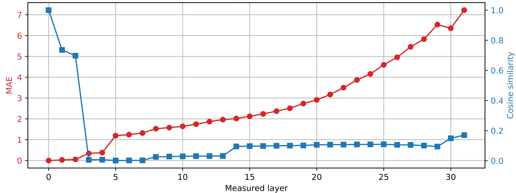
Phi-3-mini-4k-instruct | Prompt 2 Spared layer 14 | Hybrid vs unquantized
