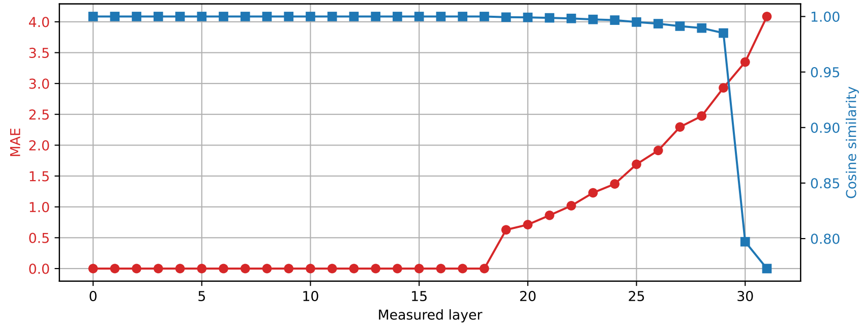
Phi-3-mini-4k-instruct | Prompt 2 Spared layer 18 | Hybrid vs quantized
