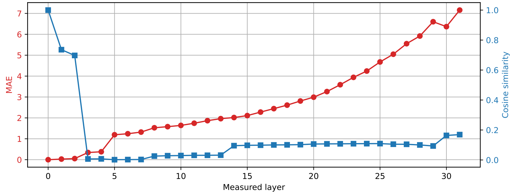
Phi-3-mini-4k-instruct | Prompt 2 Spared layer 18 | Hybrid vs unquantized
