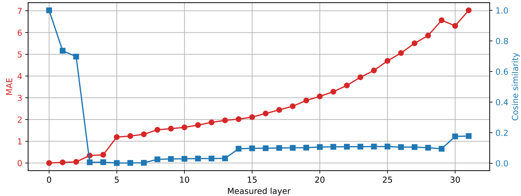
Phi-3-mini-4k-instruct | Prompt 2 Spared layer 20 | Hybrid vs unquantized
