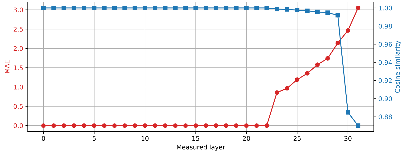
Phi-3-mini-4k-instruct | Prompt 2 Spared layer 22 | Hybrid vs quantized
