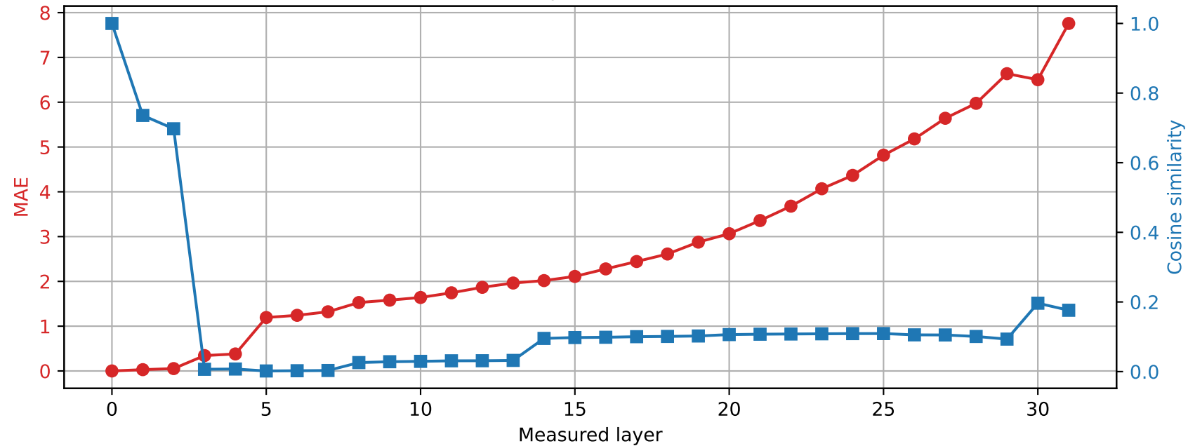
Phi-3-mini-4k-instruct | Prompt 2 Spared layer 29 | Hybrid vs unquantized
