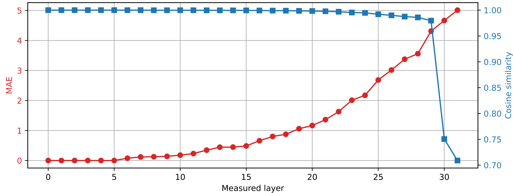
Phi-3-mini-4k-instruct | Prompt 3 Spared layer 5 | Hybrid vs quantized
