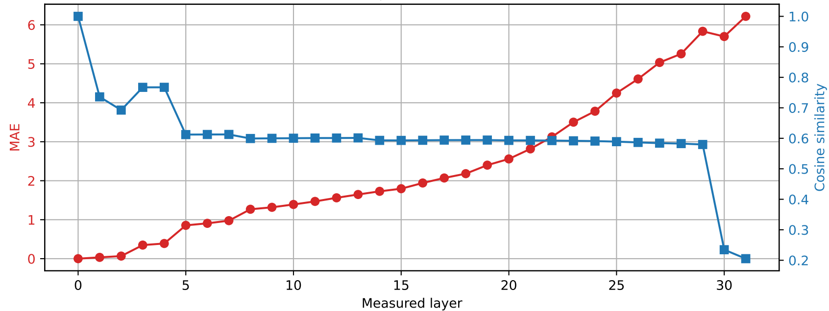
Phi-3-mini-4k-instruct | Prompt 3 Spared layer 7 | Hybrid vs unquantized
