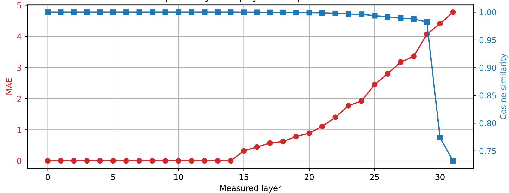
Phi-3-mini-4k-instruct | Prompt 3 Spared layer 14 | Hybrid vs quantized
