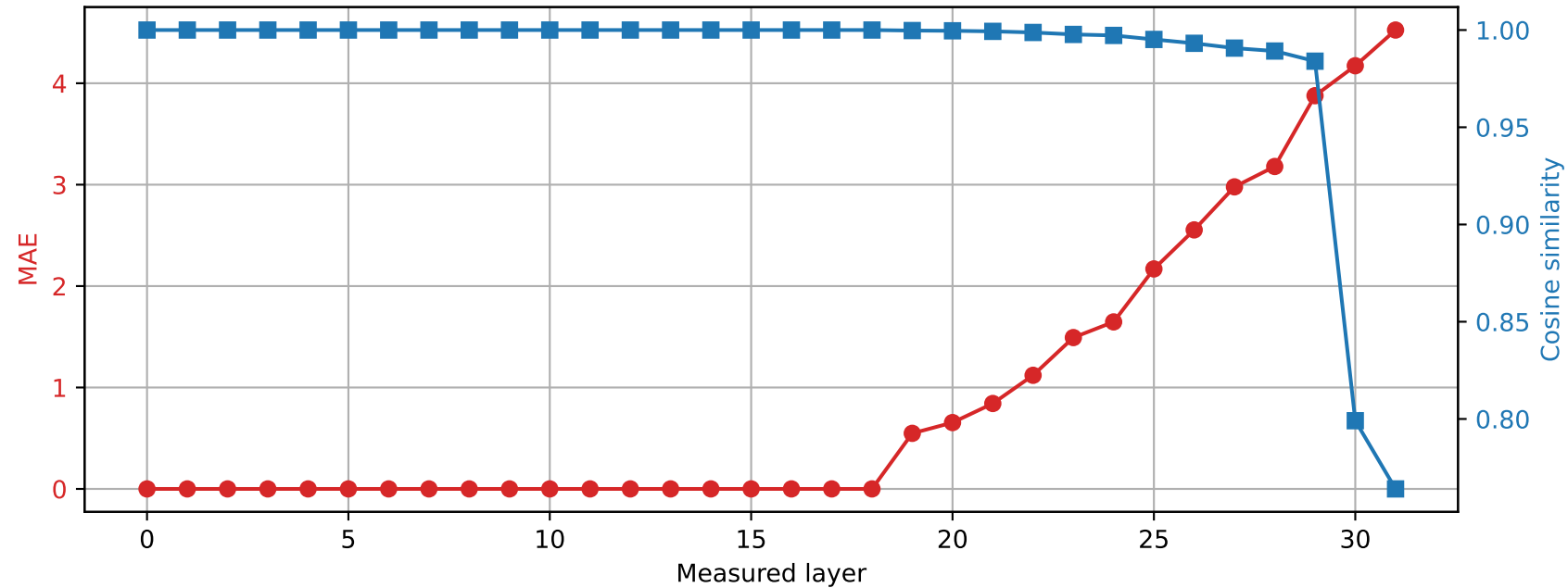
Phi-3-mini-4k-instruct | Prompt 3 Spared layer 18 | Hybrid vs quantized
