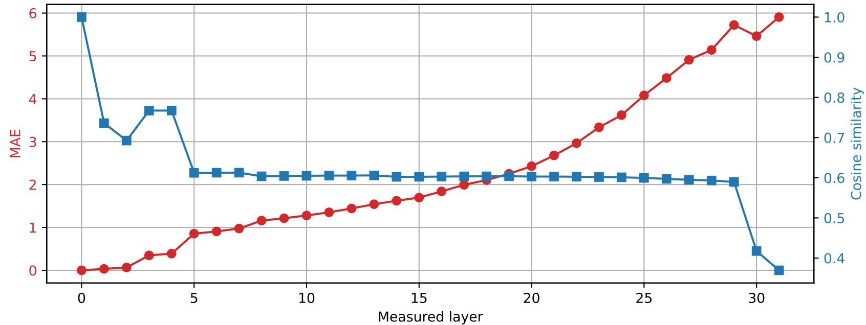
Phi-3-mini-4k-instruct | Prompt 3 Spared layer 18 | Hybrid vs unquantized
