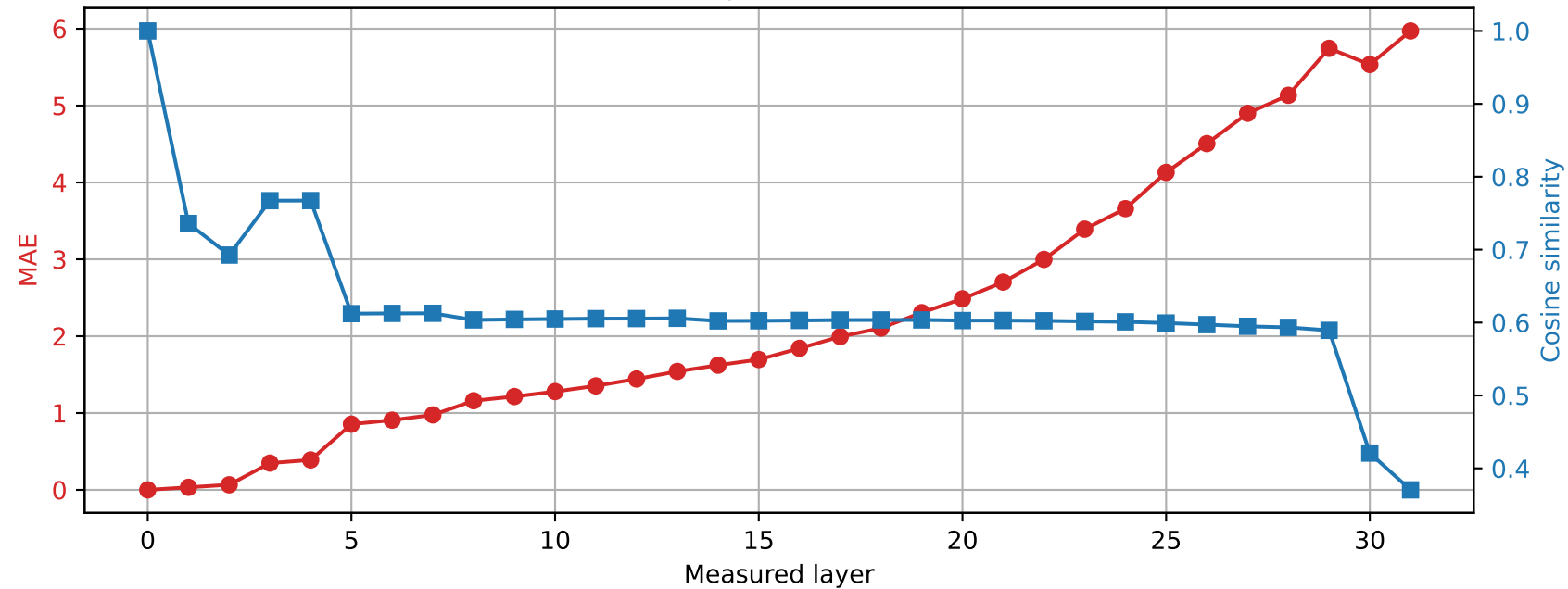
Phi-3-mini-4k-instruct | Prompt 3 Spared layer 20 | Hybrid vs unquantized
