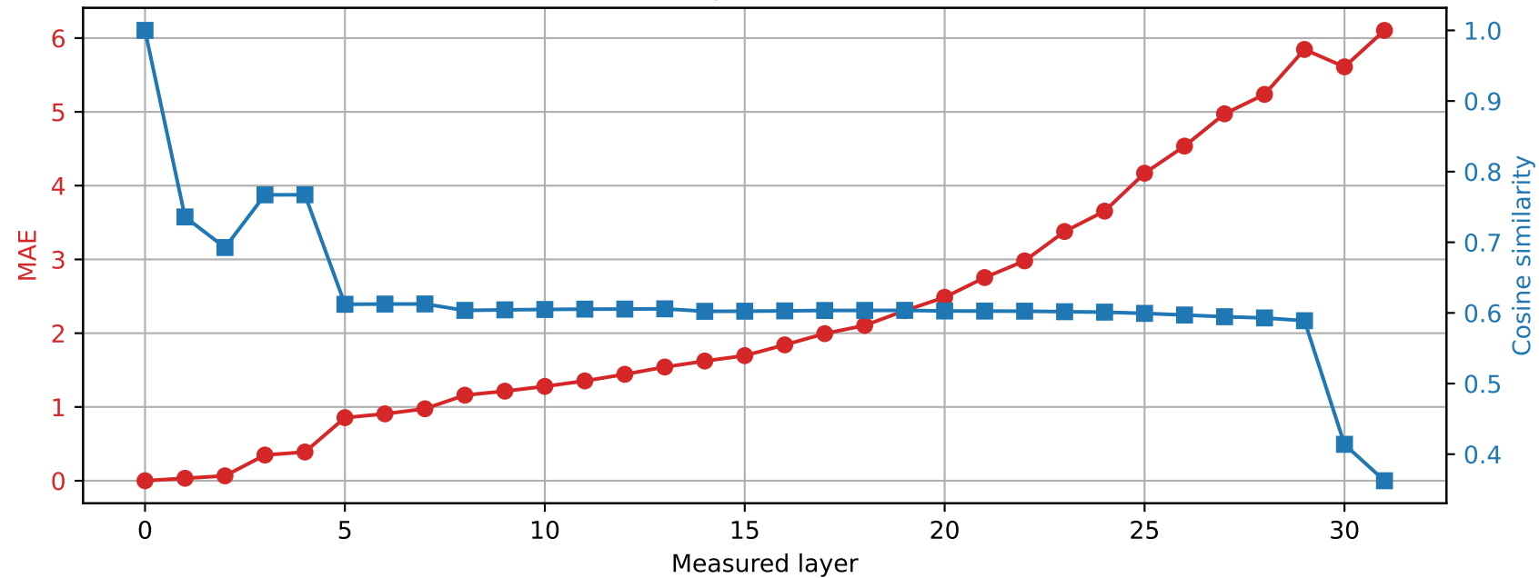
Phi-3-mini-4k-instruct | Prompt 3 Spared layer 21 | Hybrid vs unquantized
