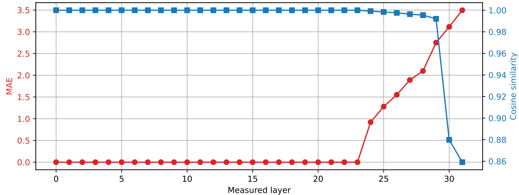
Phi-3-mini-4k-instruct | Prompt 3 Spared layer 23 | Hybrid vs quantized
