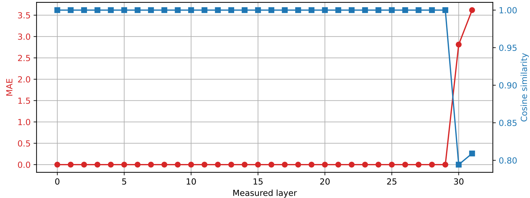
Phi-3-mini-4k-instruct | Prompt 3 Spared layer 29 | Hybrid vs quantized
