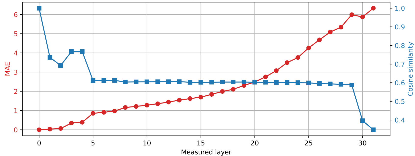
Phi-3-mini-4k-instruct | Prompt 3 Spared layer 31 | Hybrid vs unquantized
