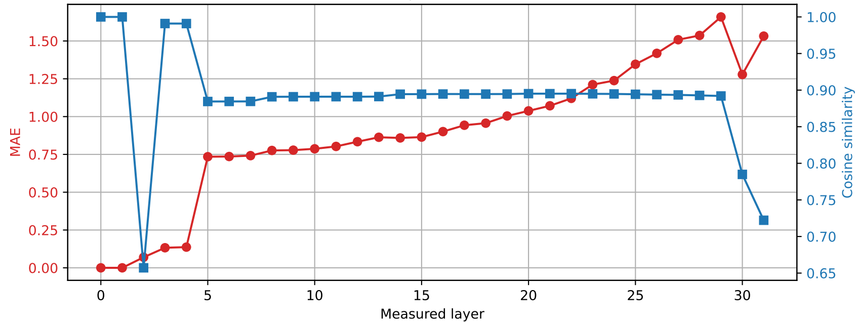
Phi-3-mini-4k-instruct | Prompt 4 Spared layer 1 | Hybrid vs quantized
