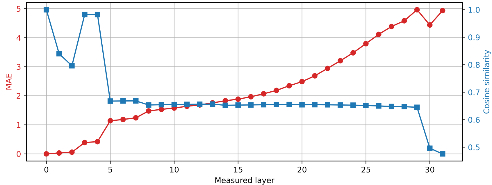
Phi-3-mini-4k-instruct | Prompt 4 Spared layer 5 | Hybrid vs unquantized
