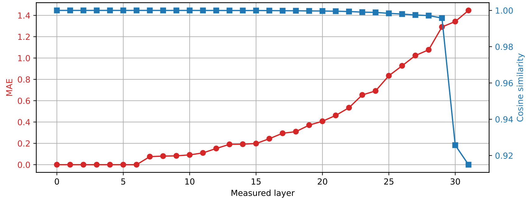
Phi-3-mini-4k-instruct | Prompt 4 Spared layer 6 | Hybrid vs quantized
