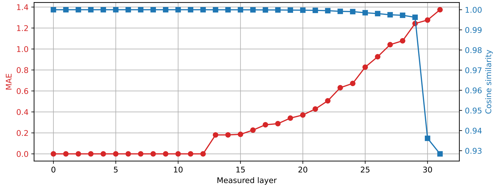
Phi-3-mini-4k-instruct | Prompt 4 Spared layer 12 | Hybrid vs quantized
