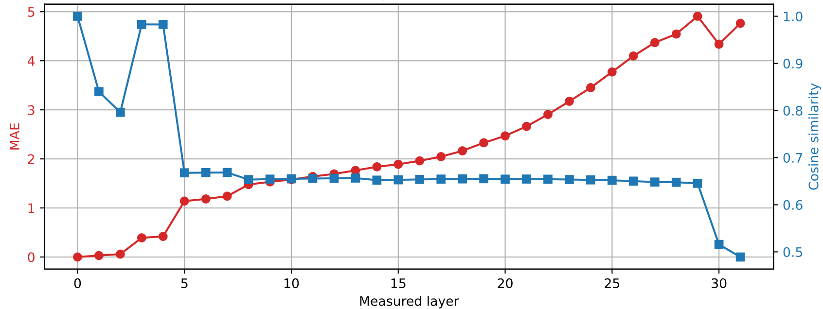
Phi-3-mini-4k-instruct | Prompt 4 Spared layer 15 | Hybrid vs unquantized
