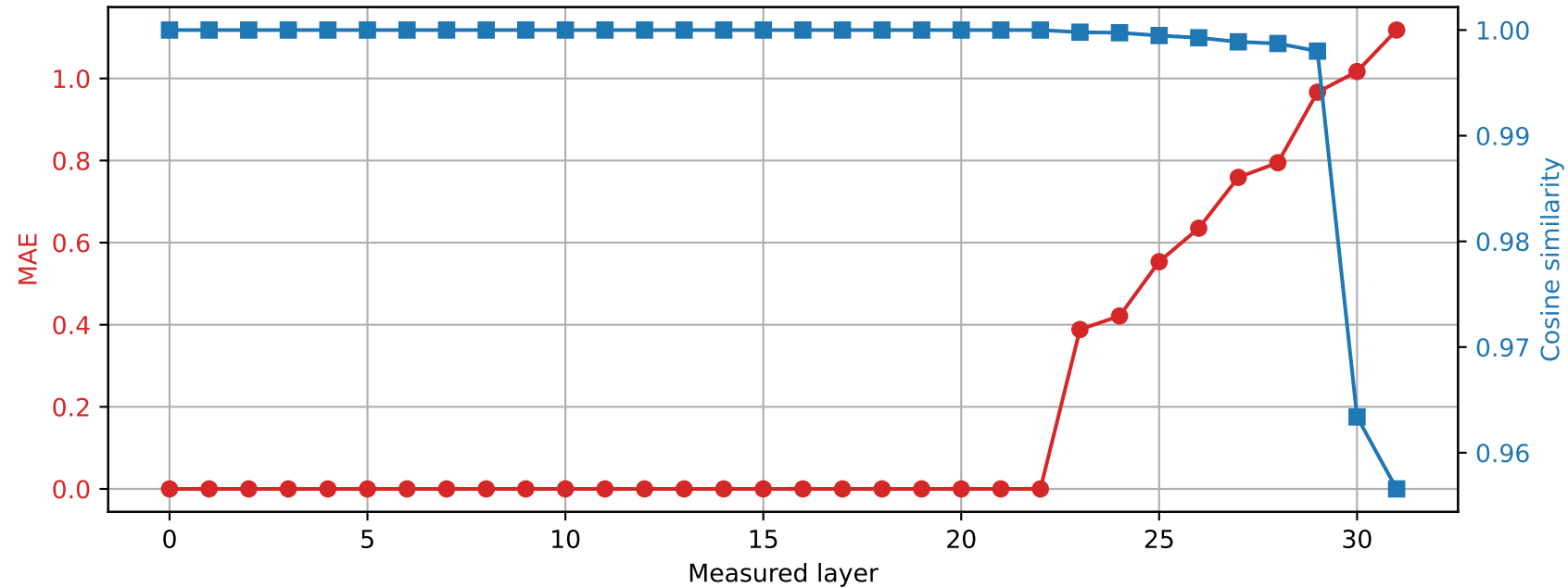
Phi-3-mini-4k-instruct | Prompt 4 Spared layer 22 | Hybrid vs quantized
