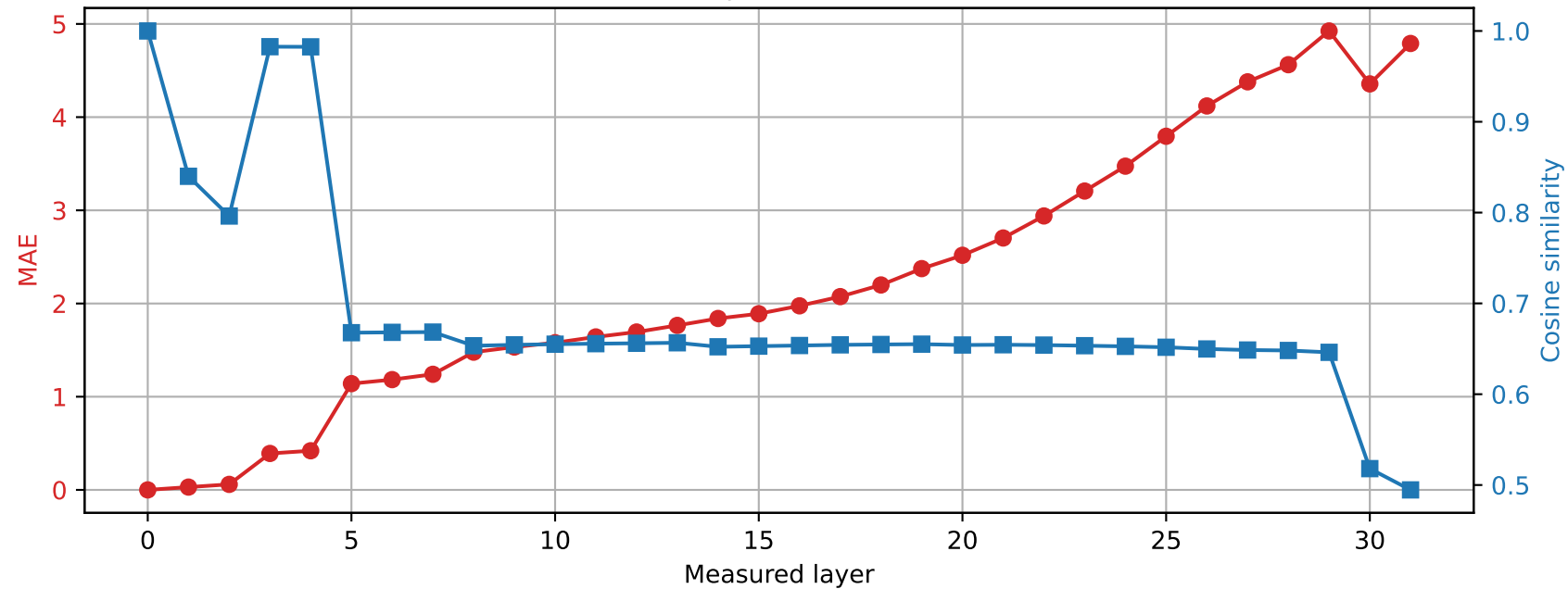
Phi-3-mini-4k-instruct | Prompt 4 Spared layer 26 | Hybrid vs unquantized
