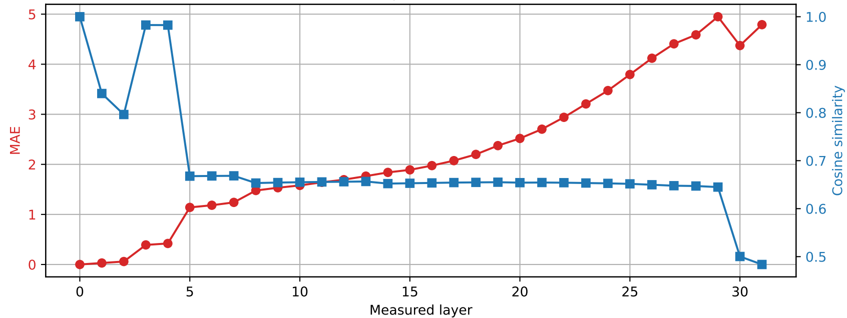
Phi-3-mini-4k-instruct | Prompt 4 Spared layer 31 | Hybrid vs unquantized
