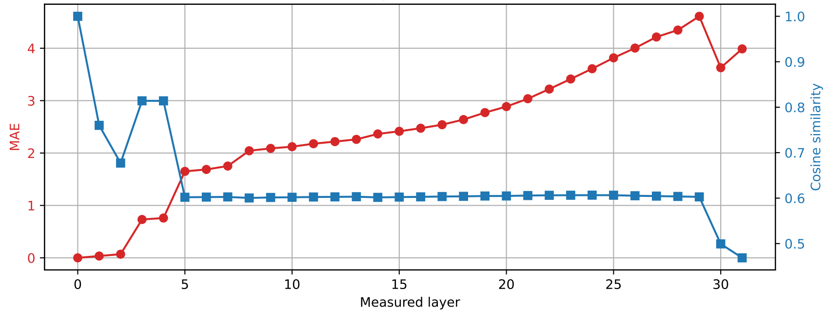
Phi-3-mini-4k-instruct | Prompt 0 Spared layer 11 | Hybrid vs unquantized
