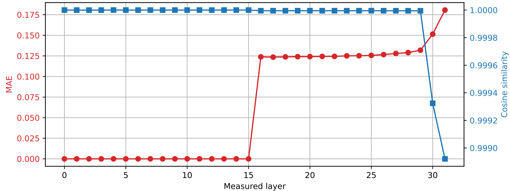
Phi-3-mini-4k-instruct | Prompt 0 Spared layer 15 | Hybrid vs quantized
